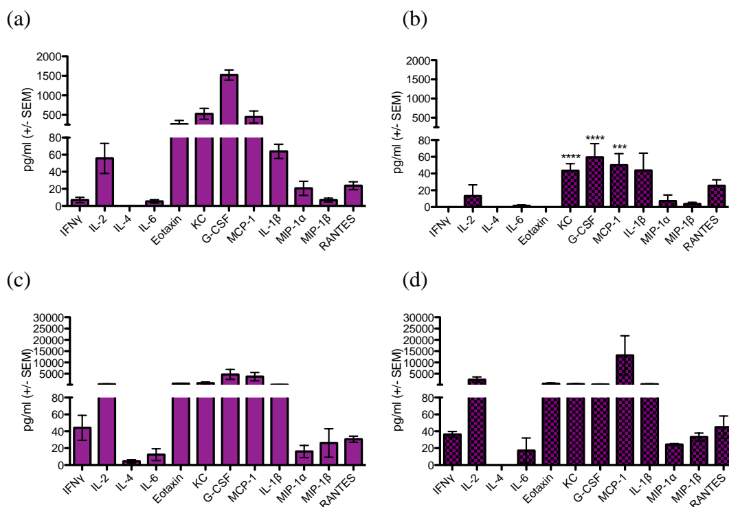
Figure 4.8. Serum cytokine levels after first protein boost in wildtype or MyD88 deficient mice vaccinated with DP6-001 and ISCOMATRIX TM adjuvant in the presence or absence of DNA priming. In the absence of DNA priming, wildtype (solid) and MyD88 deficient (checked) mice were immunized with two DP6-001 protein boosts and ISCOMATRIX TM adjuvant (a-b). DNA primed wildtype and MyD88 deficient mice were immunized with DP6-001 DNA prime-protein boost and ISCOMATRIX TM adjuvant (c-d). Sera were collected pre-immunization and 6 hours following both protein-adjuvant boosts. Cytokines were quantified in the serum of individual mice at a 1:4 dilution using a custom 12-plex Luminex panel. Shown are serum cytokine panels in (a) wildtype and (b) MyD88 deficient mice immunized with DP6-001 protein formulated with ISCOMATRIX TM adjuvant, or (c) wildtype and (d) MyD88 deficient mice immunized with DP6-001 DNA prime-protein boost formulated with ISCOMATRIX TM adjuvant. Statistical significance was determined with a One-way ANOVA and Tukey post-test (*: p < .05, **: p < .01, ***: p < .001).
